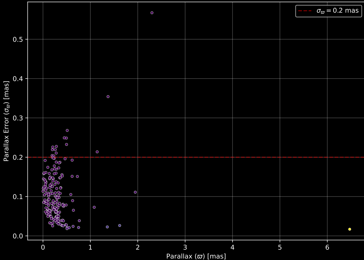
APOGEE DR17 Field: [345-02] Parallax Quality (n= 196)
