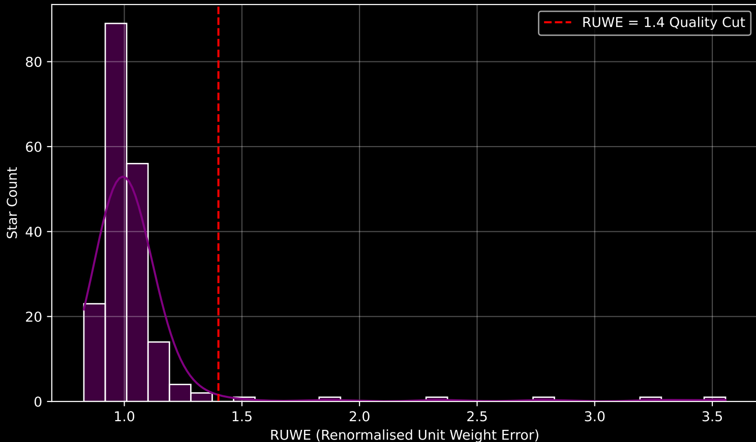
GAPOGEE DR17 Field [345-02] RUWE Distribution (n= 194)
