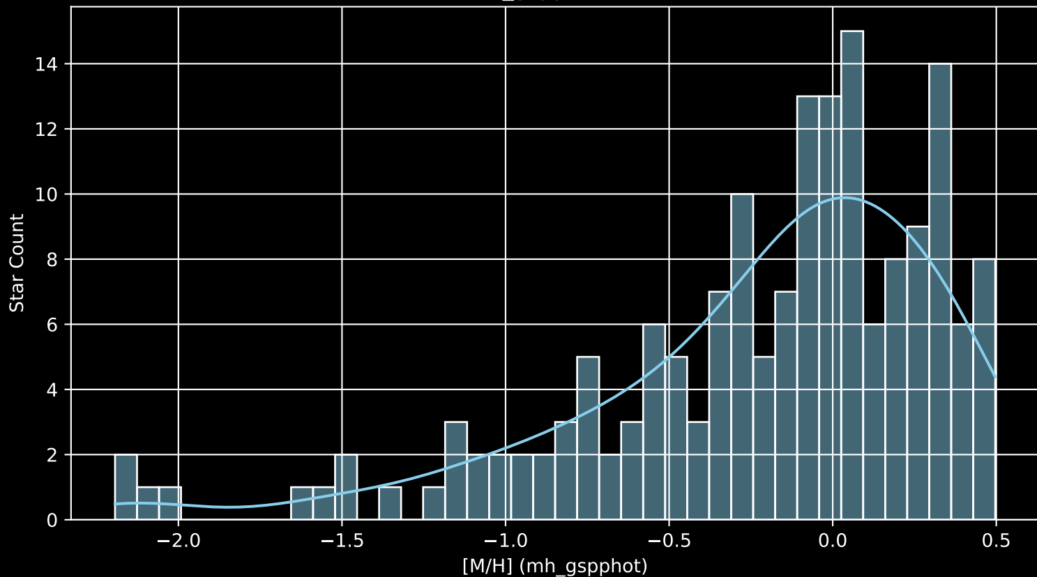
APOGEE DR17 Field: [345-02 [M/H] (mh_gspphot) (n= 169)
