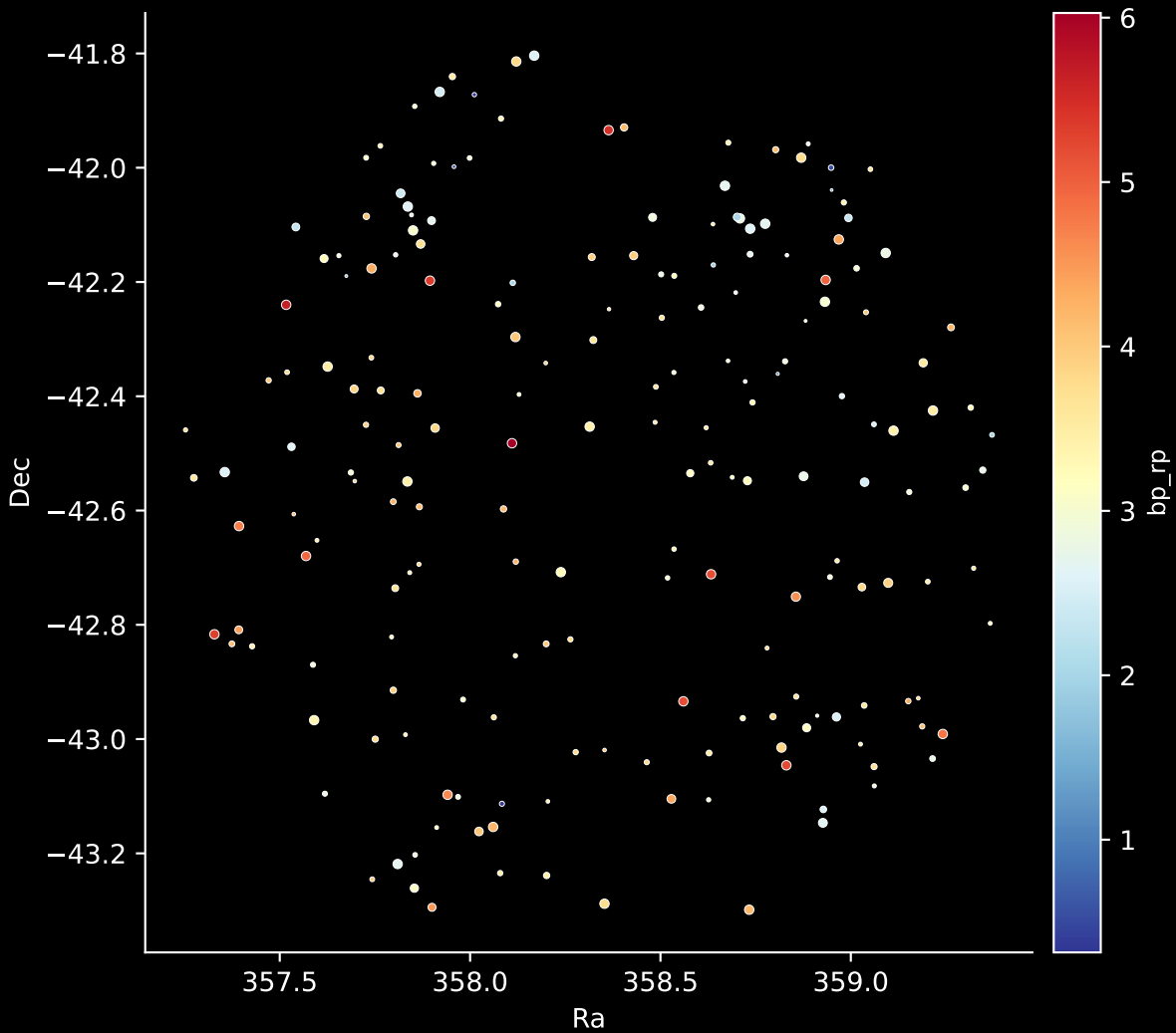
APOGEE DR17 Field: [345-02] Stars: 196
