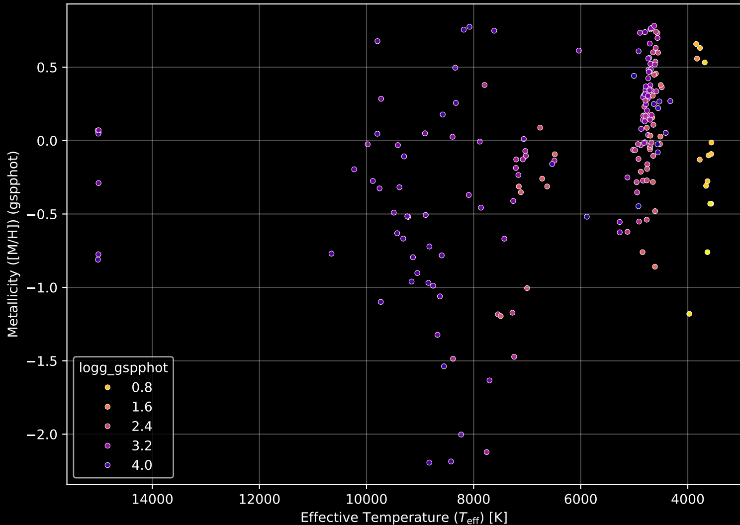
APOGEE DR17 Field: [345-02] Stellar Population Parameters (n= 196)
