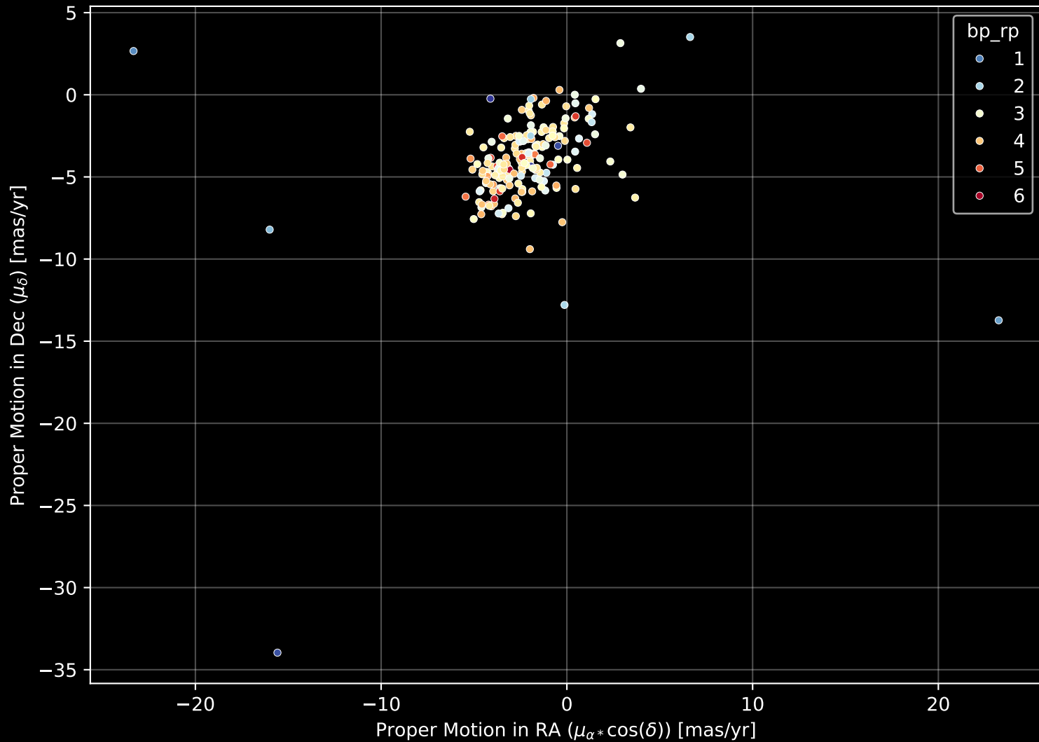
APOGEE DR17 Field: [345-02] Proper Motion Diagram (n= 196)
